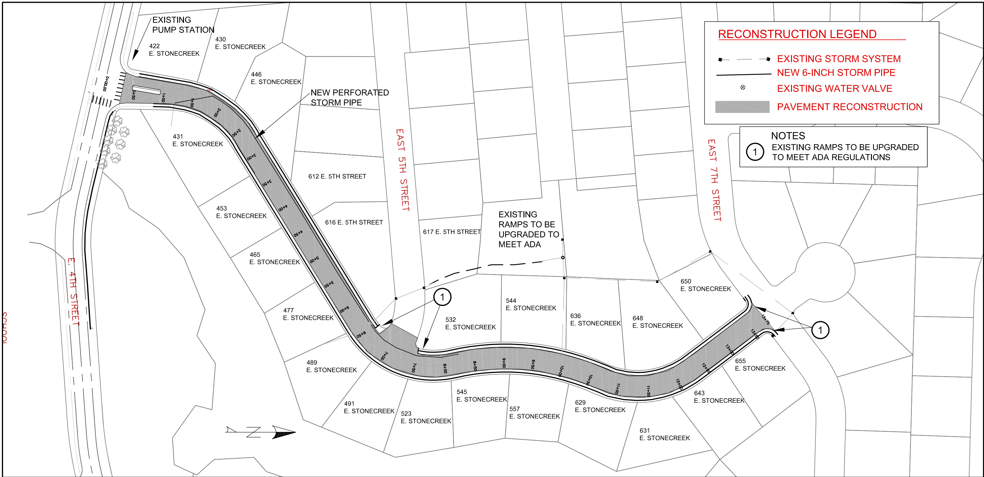
SCHMATIC STONECREEK DR. RECONSTRUCTION
