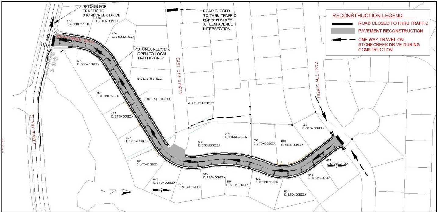
SCHEMATIC STONECREEK DR. RECONSTRUCTION
