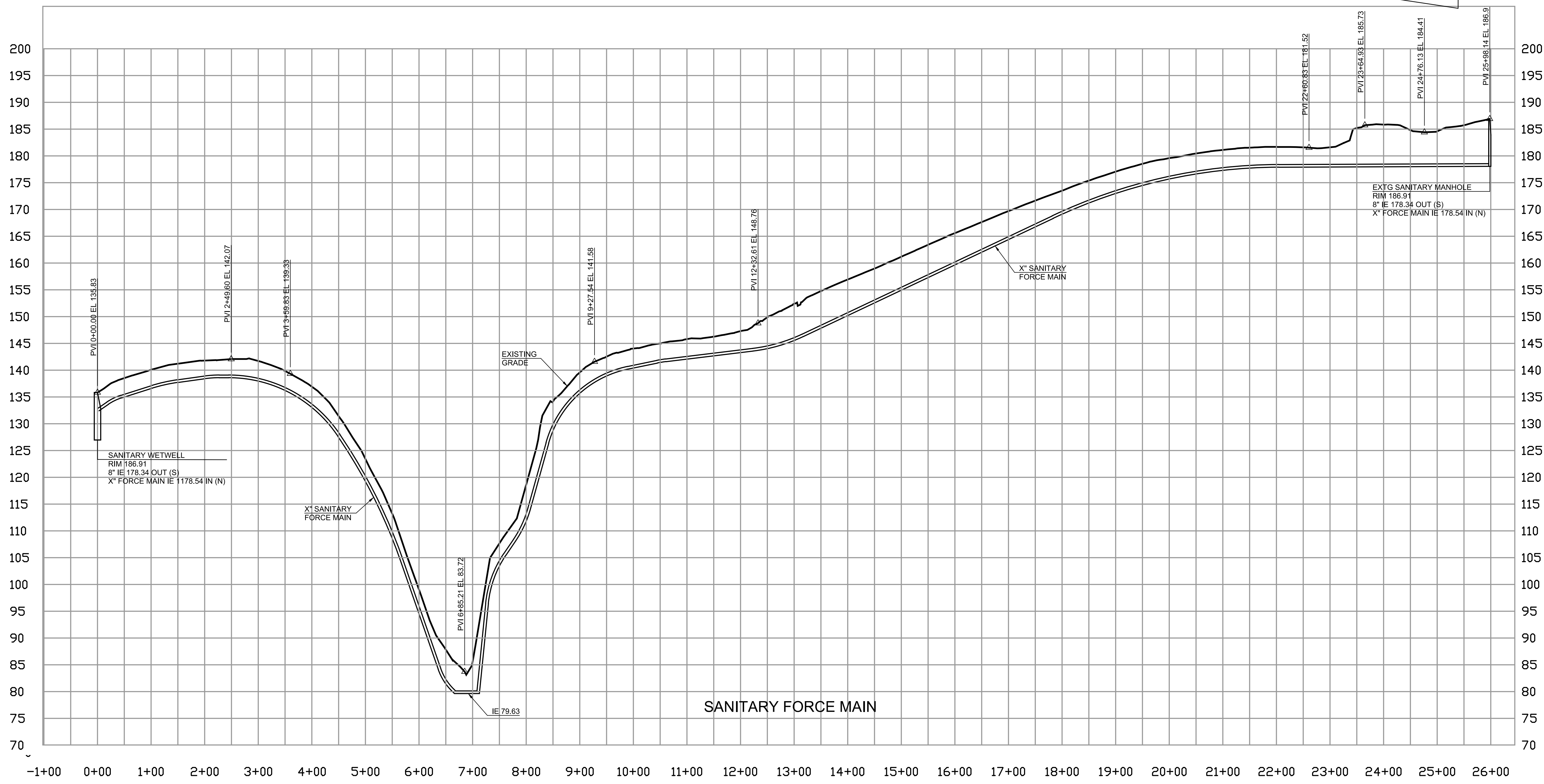
SANITARY SEWER FORCE MAIN
